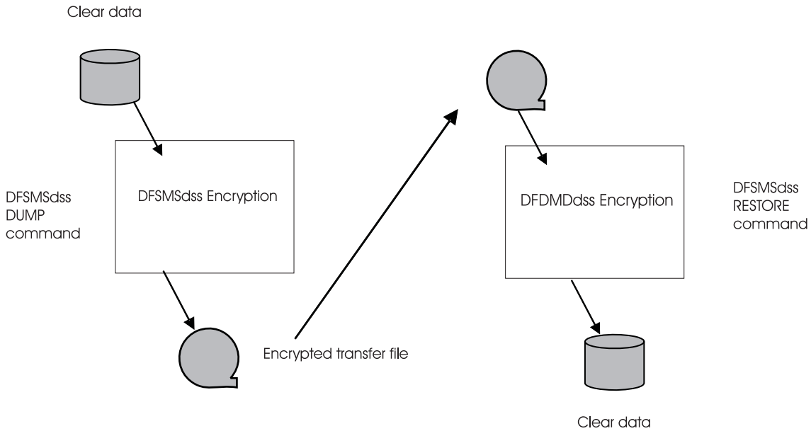
Figure 2. Encrypting and decrypting data with DFSMSdss Encryption
